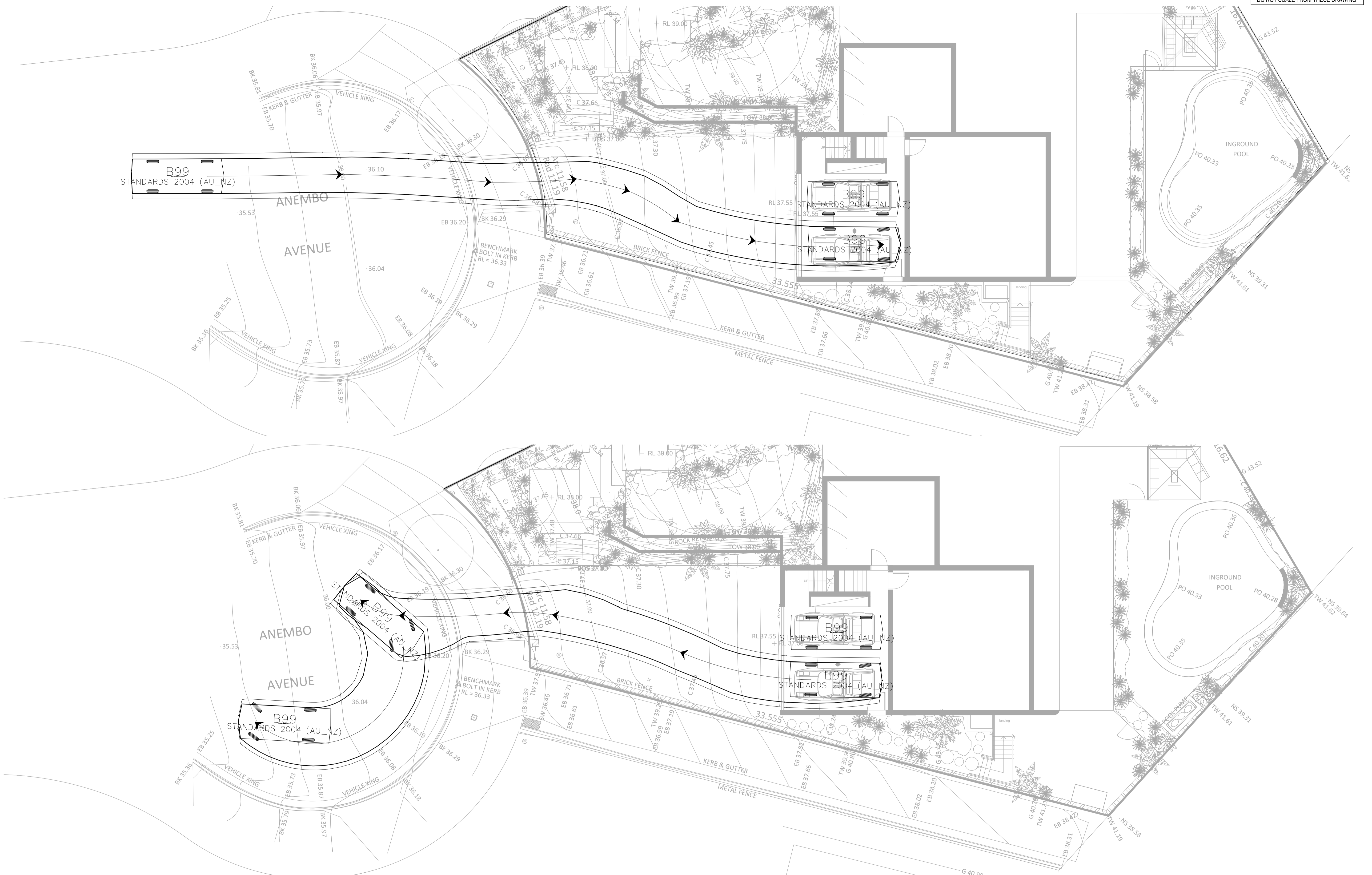
TURNING PATH ANALYSIS SCALE 1:100
