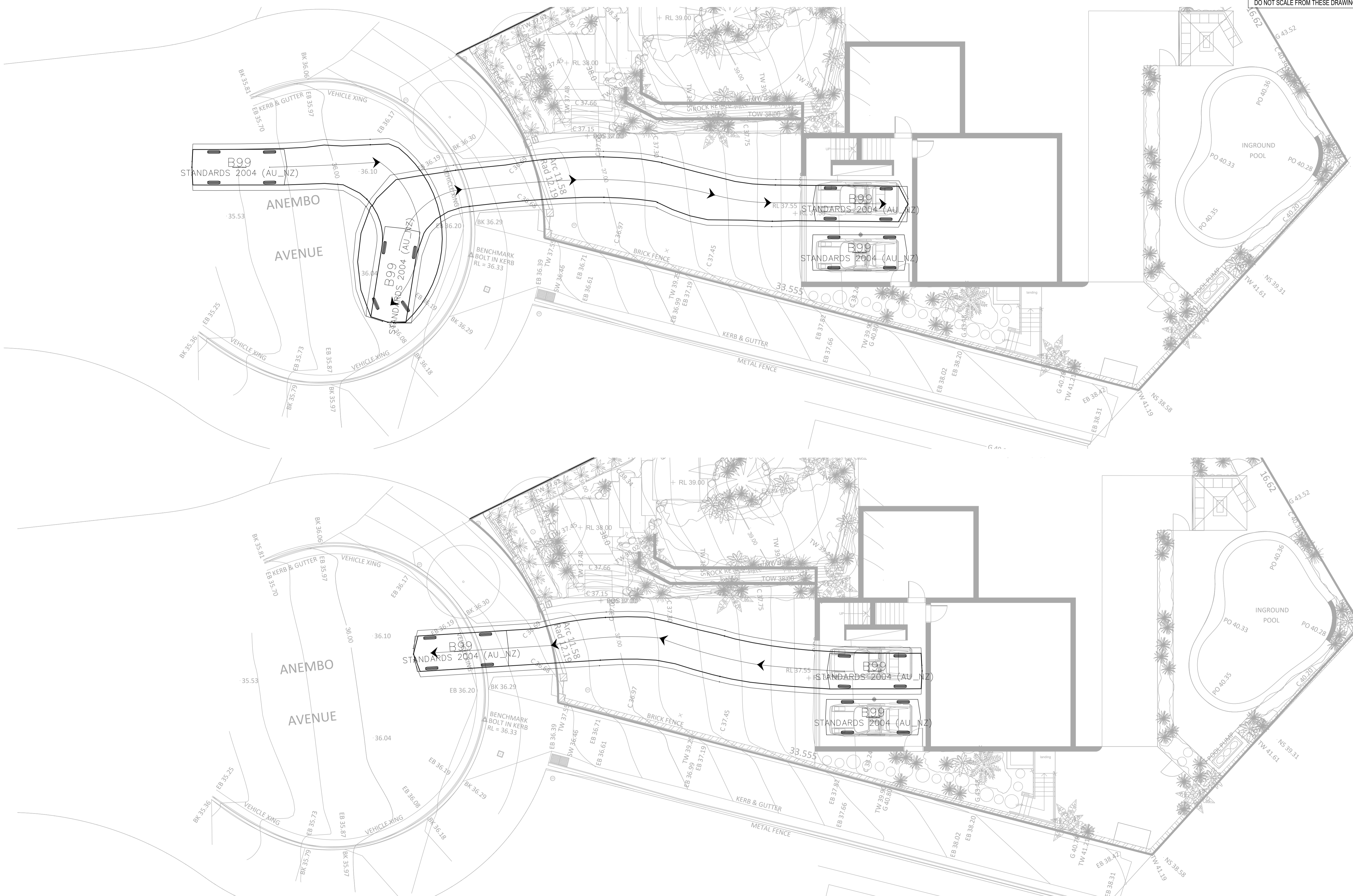
TURNING PATH ANALYSIS SCALE 1:100
